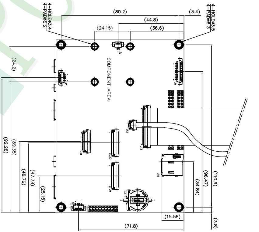
Detail SBC Board Scale 1X
