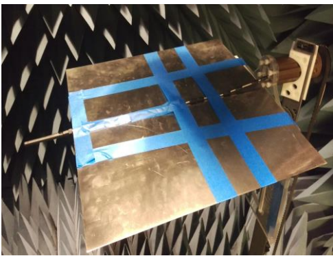
50cm x 50cm Ground Plane Edge
