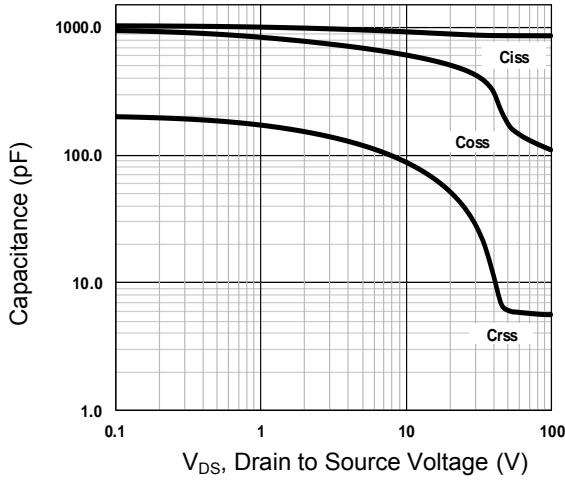
Figure 7. Capacitance Characteristics
