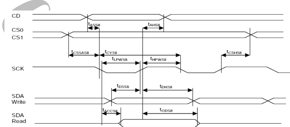
FIGURE 2 : Serial Bus Timing Characteristics (for S8)
