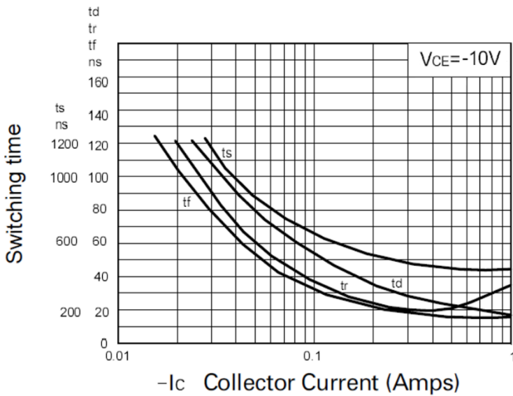
Switching Speeds
