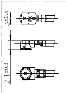
Detail B Scale:4:1
