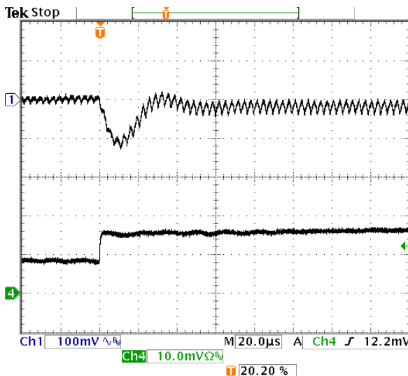
Fig-1.8V-6: Output voltage response for V_{out}=1.8V to positive load current step-change from 4A to 8A with slew rate of 5A/\mu s at V_{in}=5.0V . C_o=47\mu F \times 2 ceramic + 1\mu F ceramic. Top trace: output voltage (100mV/div.) Bottom trace: load current (5A/div.) Time scale: 20μs/div.
