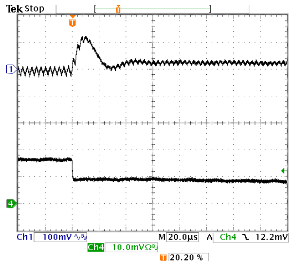
Fig-2.5V-7: Output voltage response for V_{out}=2.5V to positive load current step-change from 8A to 4A with slew rate of -5A/\mu s at V_{in}=5.0V . C_o=47\mu F \times 2 ceramic + 1\mu F ceramic. Top trace: output voltage (100mV/div.) Bottom trace: load current (5A/div.) Time scale: 20\mu s /div.
