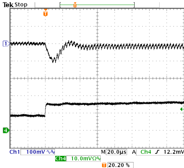
Fig-1.2V-6: Output voltage response for V_{out}=1.2V to positive load current step-change from 4A to 8A with slew rate of 5A/\mu s at V_{in}=5.0V . C_o=47\mu F \times 2 ceramic + 1\mu F ceramic. Top trace: output voltage (100mV/div.) Bottom trace: load current (5A/div.) Time scale: 20µs/div.
