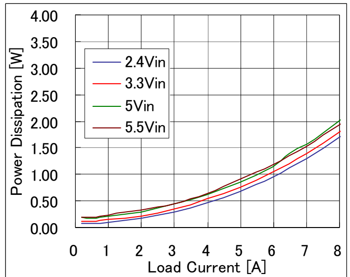
Fig-0.7525V-3: Power dissipation vs. load current and input voltage for V_{out}=0.7525V . Airflow rate=200 LFM (1.0m/s) and T_a=25^{\circ}C .
