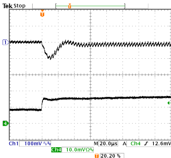
Fig-0.7525V-6: Output voltage response for V_{out}=0.7525V to positive load current step-change from 4A to 8A with slew rate of 5A/\mu s at V_{in}=5.0V . C_o=47\mu F \times 2 ceramic + 1\mu F ceramic.
