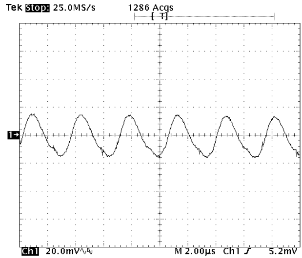
Fig-3.3V-5: Output voltage ripple (20mV/div.) for V_{out}=3.3V at full rated load current into a resistive load with external capacitance 47\mu F \times 2 ceramic + 1µF ceramic at V_{in}=5.0V . Time scale: 2µs/div
