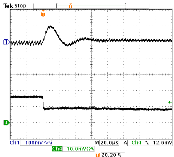
Fig-0.7525V-7: Output voltage response for V_{out}=0.7525V to positive load current step-change from 8A to 4A with slew rate of -5A/\mu s at V_{in}=5.0V . C_o=47\mu F \times 2 ceramic + 1\mu F ceramic.
