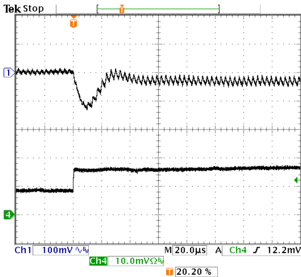
Fig-3.3V-6: Output voltage response for V_{out}=3.3V to positive load current step-change from 4A to 8A with slew rate of 5A/\mu s at V_{in}=5.0V . C_o=47\mu F \times 2 ceramic + 1µF ceramic. Top trace: output voltage (100mV/div.) Bottom trace: load current (5A/div.) Time scale: 20µs/div.
