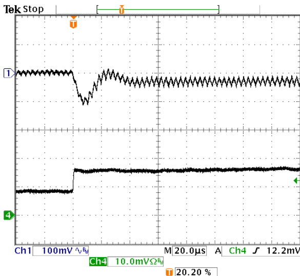
Fig-2.5V-6: Output voltage response for V_{out}=2.5V to positive load current step-change from 4A to 8A with slew rate of 5A/\mu s at V_{in}=5.0V . C_o=47\mu F \times 2 ceramic + 1\mu F ceramic. Top trace: output voltage (100mV/div.) Bottom trace: load current (5A/div.) Time scale: 20\mu s /div.
