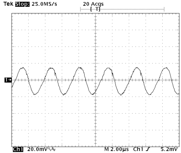
Fig-1.5V-5: Output voltage ripple (20mV/div.) for V_{out}=1.5V at full rated load current into a resistive load with external capacitance 47\mu F \times 2 ceramic + 1\mu F ceramic at V_{in}=5.0V .
