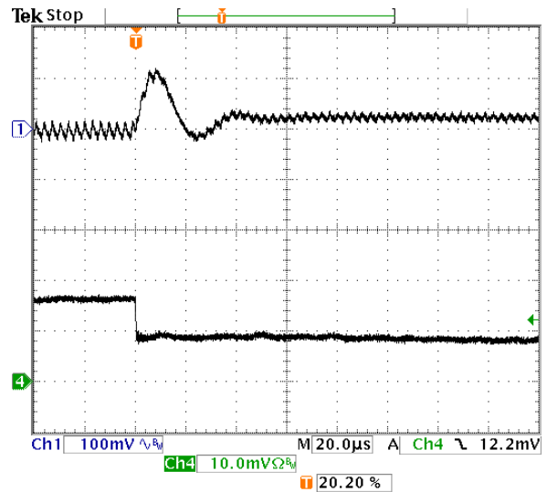
Fig-3.3V-7: Output voltage response for V_{out}=3.3V to positive load current step-change from 8A to 4A with slew rate of -5A/\mu s at V_{in}=5.0V . C_o=47\mu F \times 2 ceramic + 1µF ceramic. Top trace: output voltage (100mV/div.) Bottom trace: load current (5A/div.) Time scale: 20µs/div.
