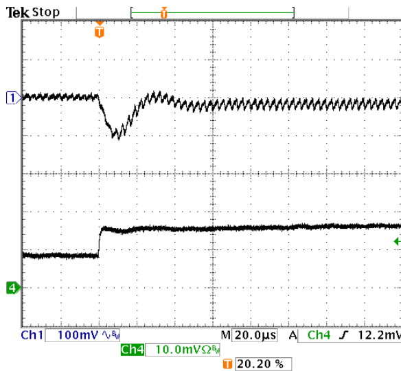
Fig-1.0V-6: Output voltage response for V_{out}=1.0V to positive load current step-change from 4A to 8A with slew rate of 5A/\mu s at V_{in}=5.0V . C_o=47\mu F \times 2 ceramic + 1\mu F ceramic.
