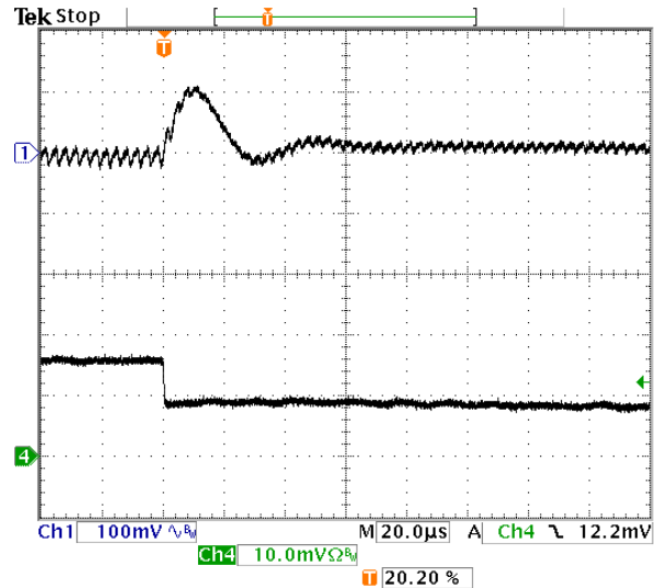
Fig-1.2V-7: Output voltage response for V_{out}=1.2V to positive load current step-change from 8A to 4A with slew rate of -5A/\mu s at V_{in}=5.0V . C_o=47\mu F \times 2 ceramic + 1\mu F ceramic. Top trace: output voltage (100mV/div.) Bottom trace: load current (5A/div.) Time scale: 20µs/div.
