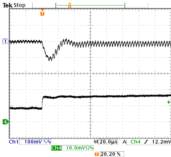
Fig-1.5V-6: Output voltage response for V_{out}=1.5V to positive load current step-change from 4A to 8A with slew rate of 5A/\mu s at V_{in}=5.0V . C_o=47\mu F \times 2 ceramic + 1\mu F ceramic.
