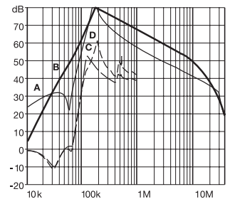
280A types
