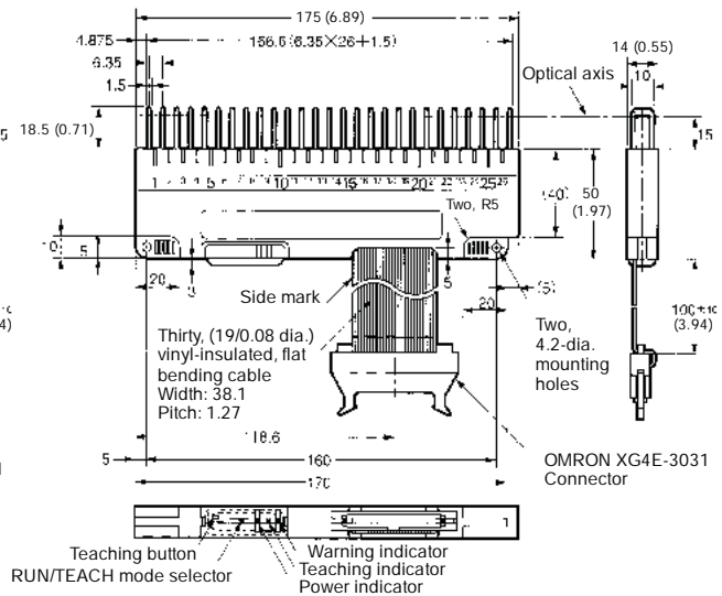
Mounting Dimensions
