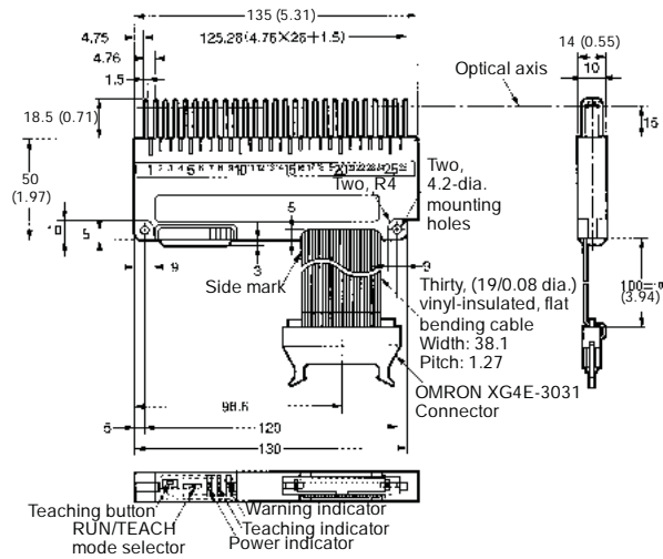
Mounting Dimensions
