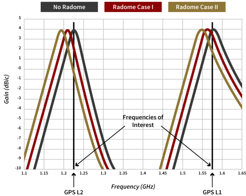
Figure 1 – Effect of Radome on Dual Frequency Antenna Gain
