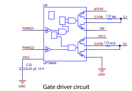
Synchronous bootstrap
