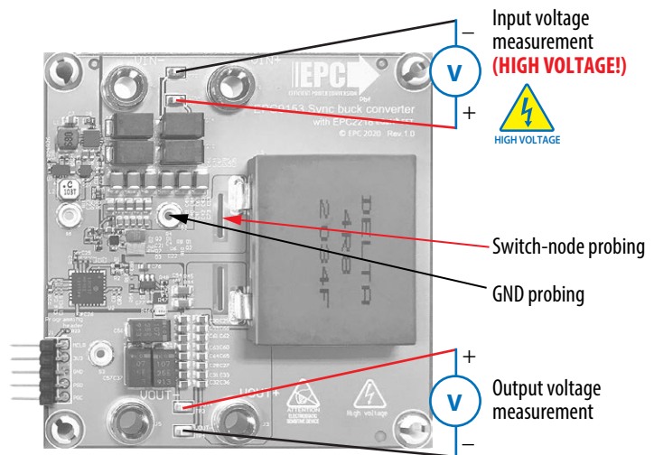
Figure 14: Measurement connection
