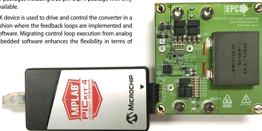
Figure 9: Programming connection
