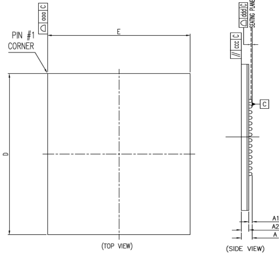
Figure 2 – Package Dimensions
