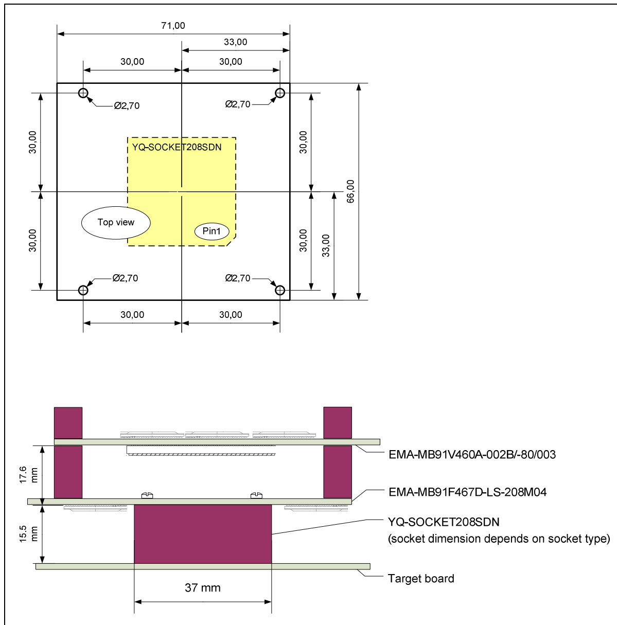
Figure 5-1: Mechanical dimensions
