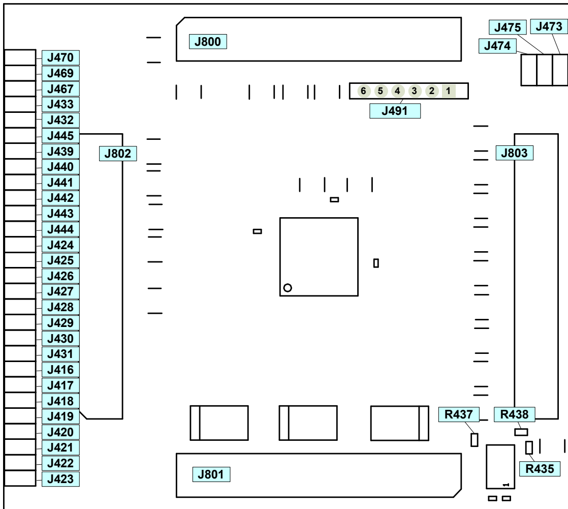
Figure 3-1: Jumper default setting, top
