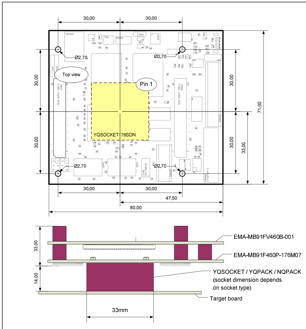
Figure 4-1: Mechanical Dimensions
