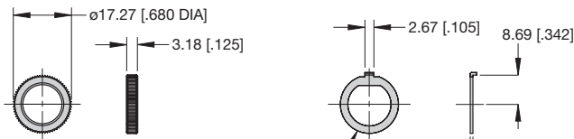
KNURLED NUT
