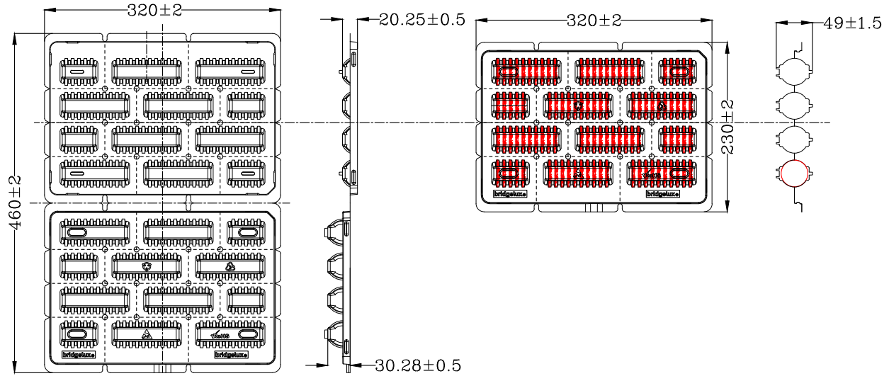
Figure 14: Packaging Specifications
