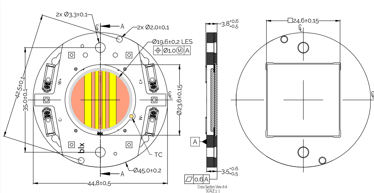
Figure 18: Mechanical Drawing Specifications
