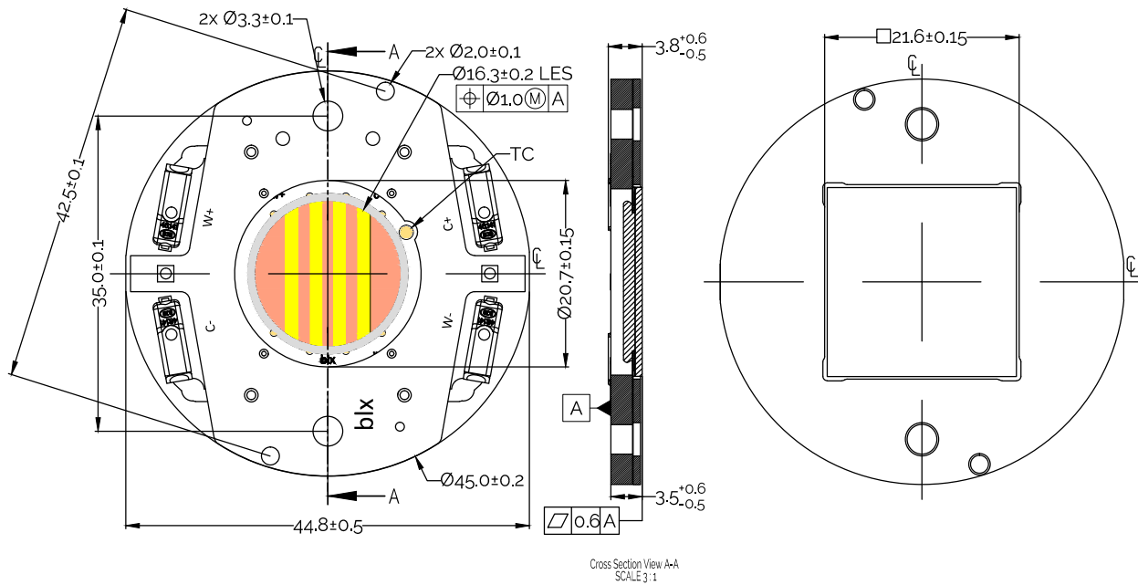
Figure 14: Mechanical Drawing Specifications
