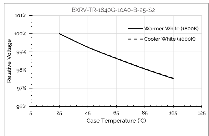
Figure 17: Relative Voltage vs. Case Temperature
