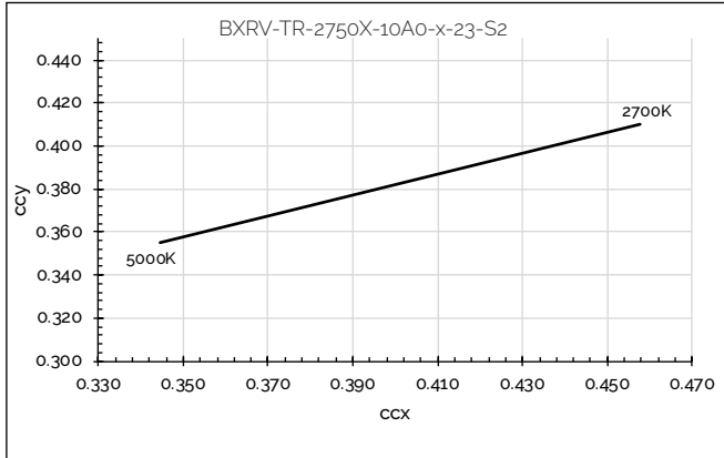
Figure 24: CCT Tuning Range, Tc=85C
