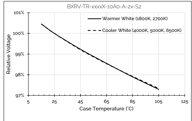
Figure 15: Relative Voltage vs. Case Temperature
