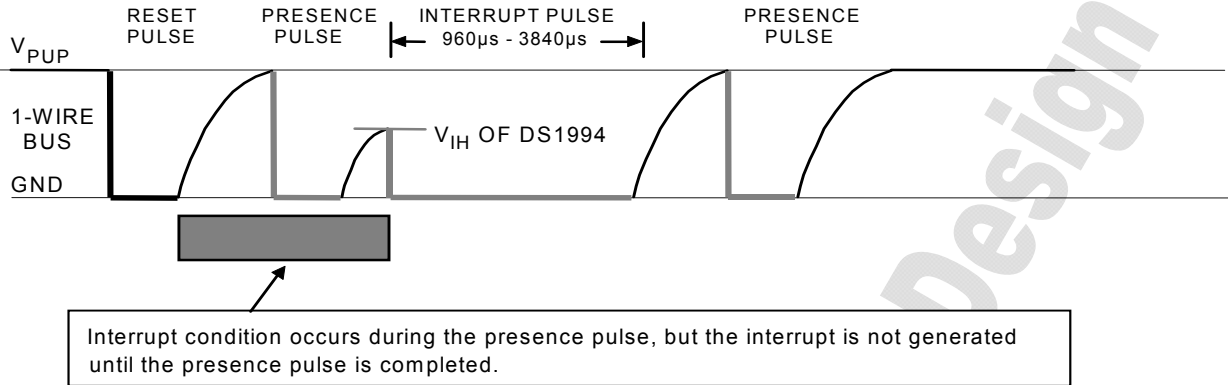
Figure 14. TYPE 2 INTERRUPT
