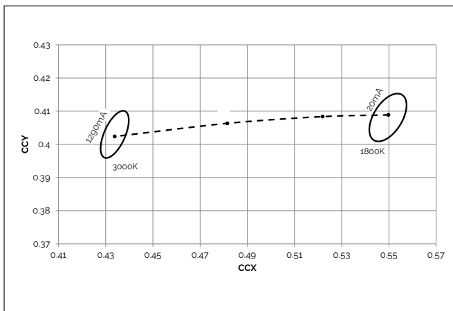
Figure 7: Color Shift vs. Forward Current 3000K-1800K, T_c=25^\circ\text{C}
