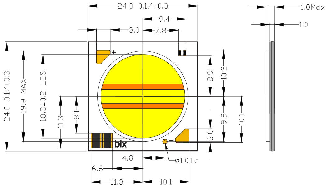
Figure 12: Mechanical Drawing Specification
