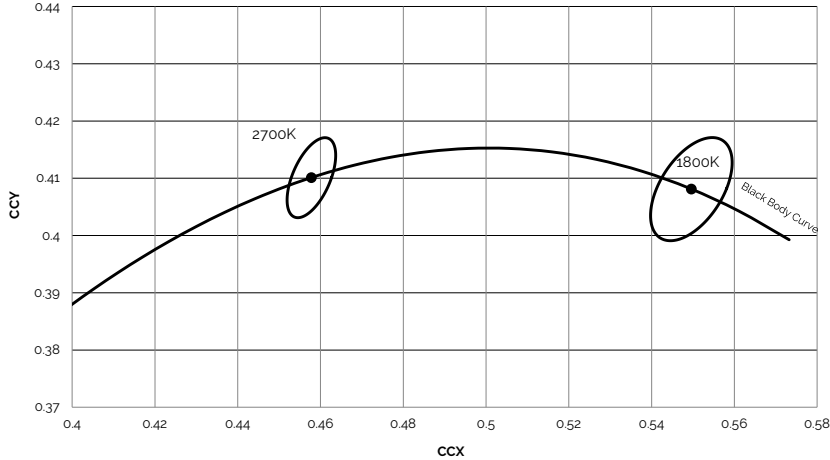
Figure 13: Graph of Warm White Test Bins in xy Color Space, T_c = 25^\circ\text{C}
