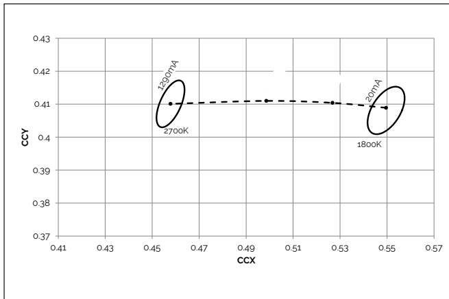
Figure 6: Color Shift vs. Forward Current 2700K-1800K, T_c=25^\circ\text{C}
