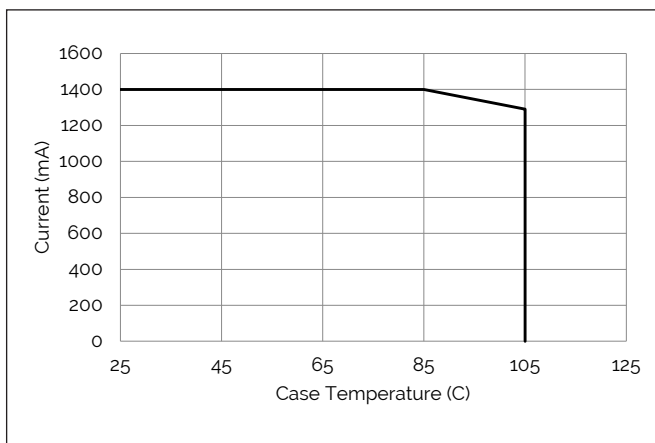
Figure 8: Derating Curve
