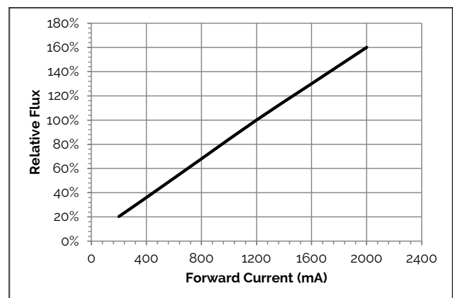
Figure 9: Flux vs. Current (1120mm only)
