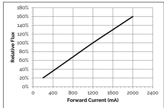
Figure 7: Flux vs. Current (560mm only)
