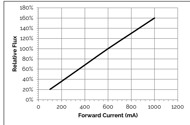
Figure 5: Flux vs. Current (280mm only)
