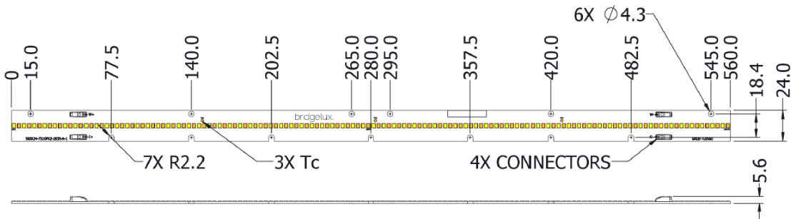
Figure 20: Drawing Overview for 560mm
