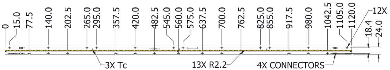
Figure 21: Drawing Overview for 1120mm
