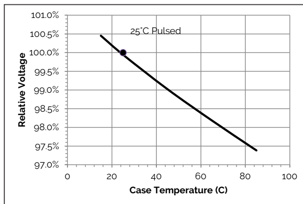
Figure 16: Voltage vs Case Temperature
