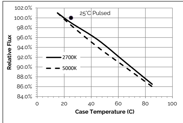
Figure 14: Flux vs Case Temperature (2700K-5000K)
