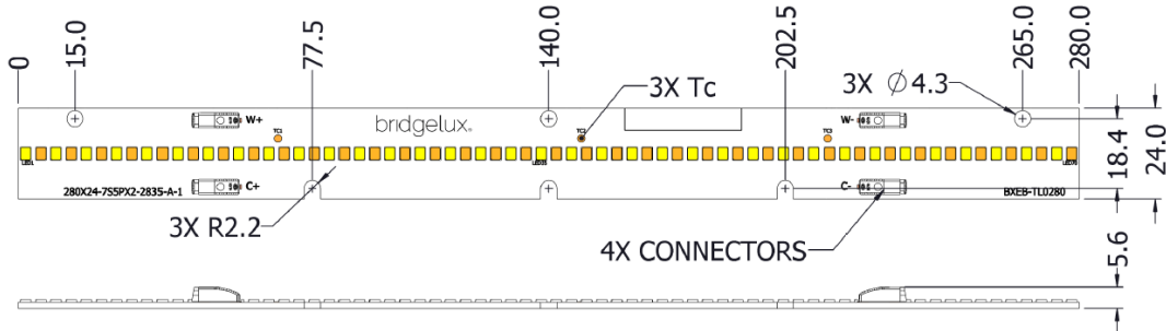
Figure 19: Drawing Overview for 280mm
