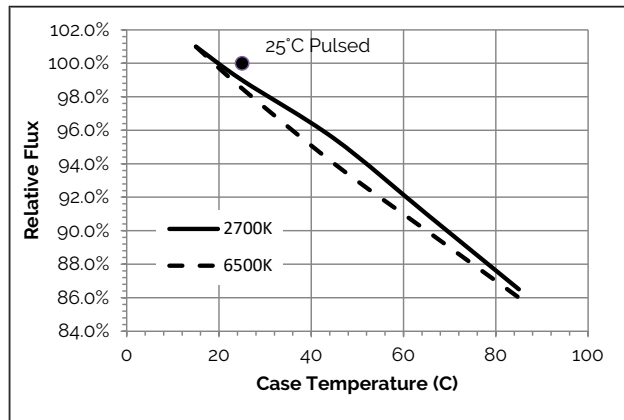
Figure 15: Flux vs Case Temperature (2700K-6500K)
