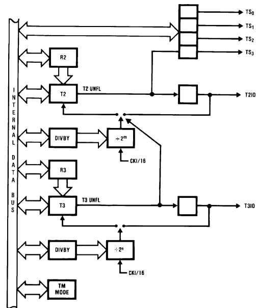
TL/DD/11372-18 FIGURE 20. Timers T2-T3 Block
