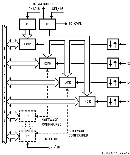
TL/DD/11372-17 FIGURE 19. Timers T0, T1 and T8 with Four Input Capture Registers
