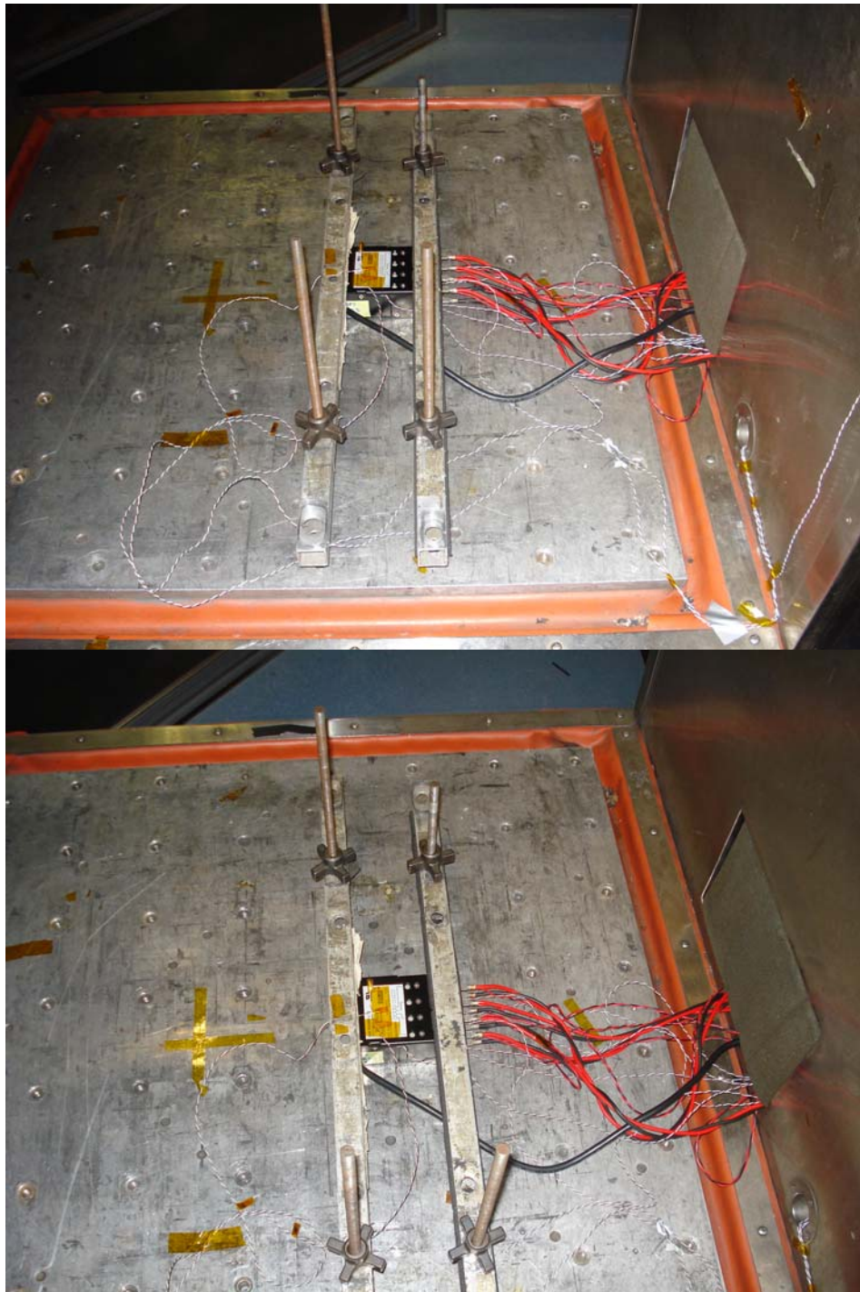
Figure 1 – Thermal and vibration Set-up
