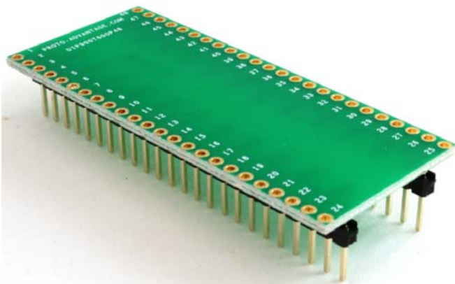
3D Top View (Pins Assembled)
