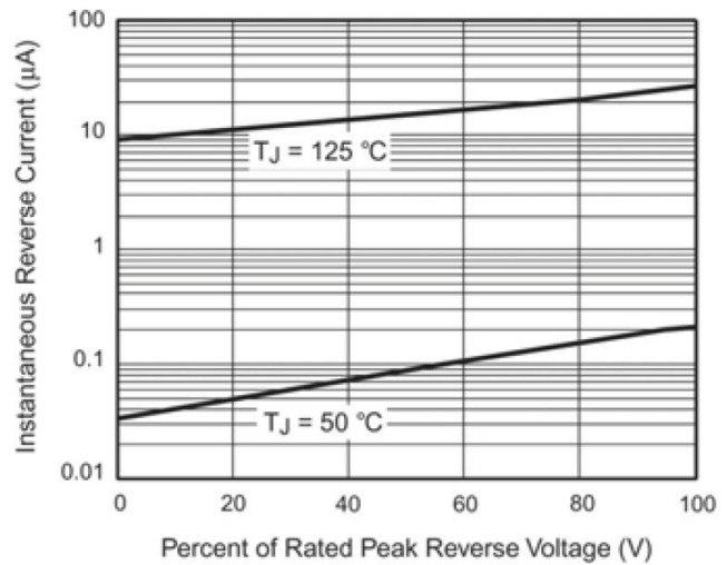
Figure 4. Typical Reverse Leakage Characteristics Per Leg
