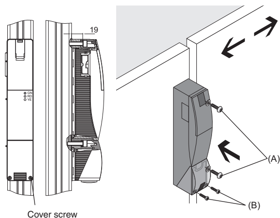
Cover screw
