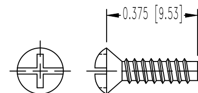
COVER SCREW 2X
