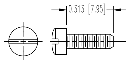
CABLE CLAMP SCREW 2X
