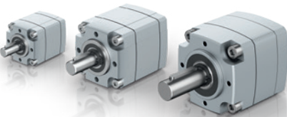
Optimax® 42.1, 63.1 and 80.1
