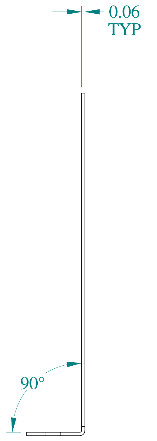
SIDE VIEW
