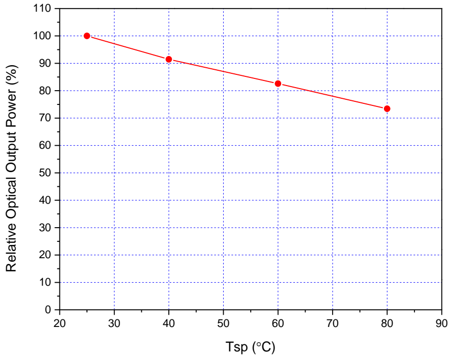
Fig 5. Relative Optical Output Power vs. Solder Point Temperature, I_F=100\text{mA}
