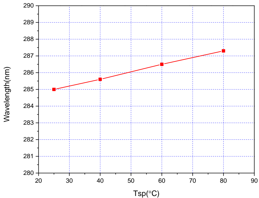
Fig 6. Peak Wavelength vs. Solder Point Temperature, I_F=100\text{mA}
