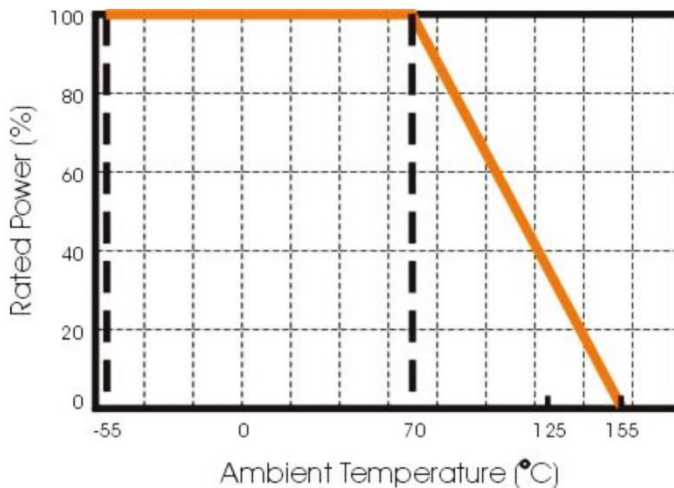
Fig 1 Maximum dissipation in percentage of rated power as a function of the ambient temperature for RCR06
