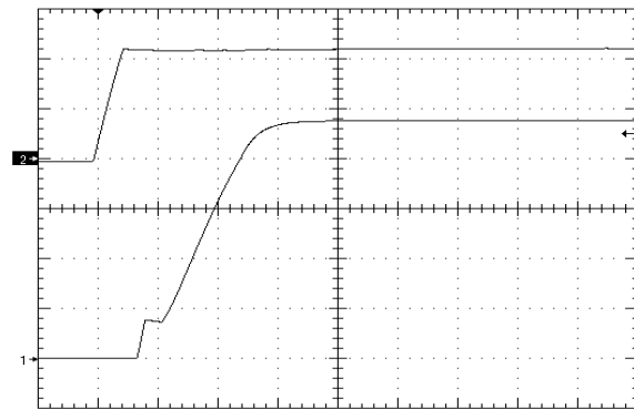
Figure 8. Startup Waveform via Line Voltage, time scale 10mS/div. Vin=Vin_nom, full res. load + 330uF, negative enbl, Ch1=5V/div, Ch2=20V/div
