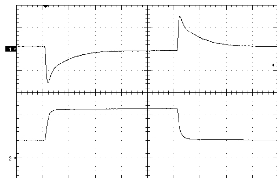
Figure 10. Load Transient Response (50mV/div), di/dt=0.1A/uS, 25% - 75% - 25% of full load time scale: 200uS/div
