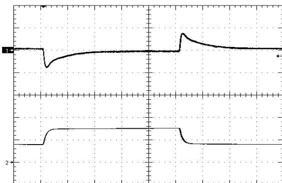
Figure 9. Load Transient Response (50mV/div), di/dt=0.05A/uS, 50% - 25% - 50% of full load, time scale: 200uS/div
