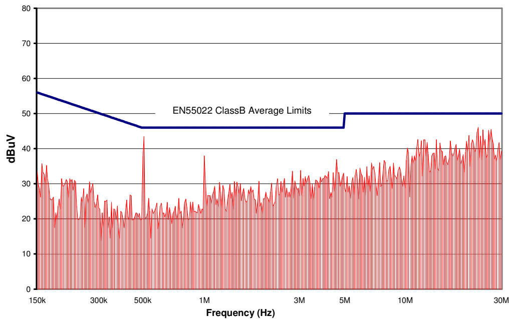
Figure 16. CPT3D48 Conducted Emissions using above specified input filter, Vin = 48V, Full Resistive Load
