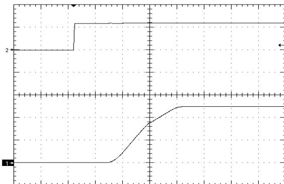
Figure 11. Startup Waveform via Enable Pin, time scale 4mS/div. Vin=Vin_nom, Iout=full load Cout=4700uF, Ch1=Vout (2V/div), Ch2=Enable (5V/div)
