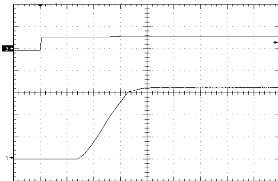
Figure 11. Startup Waveform via Enable Pin, time scale 2mS/div. Vin=Vin_nom, Iout=no load Cout=4700uF, Ch1=Vout (1V/div), Ch2=enable (10V/div)
