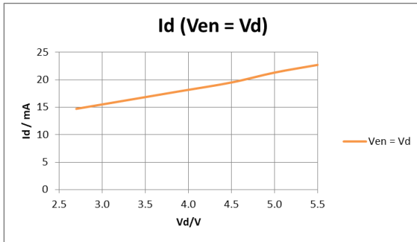
Figure 32: Id (Ven = Vd)
