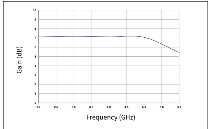
Figure 8. Power Gain vs Frequency of the CGH40006P in the CGH40006P-AMP P_{IN} = 30 \text{ dBm} , V_{DD} = 20 \text{ V}
