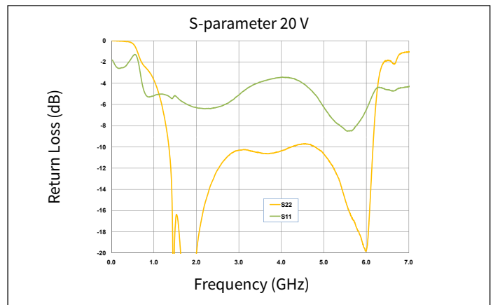
Figure 4. Input & Output Return Losses vs Frequency at 20 V of the CGH40006P in the CGH40006P-AMP
