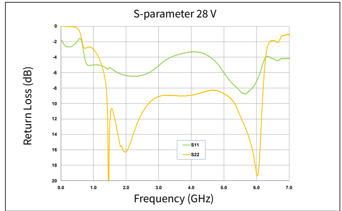
Figure 2. Input & Output Return Losses vs Frequency at 28 V of the CGH40006P in the CGH40006P-AMP
