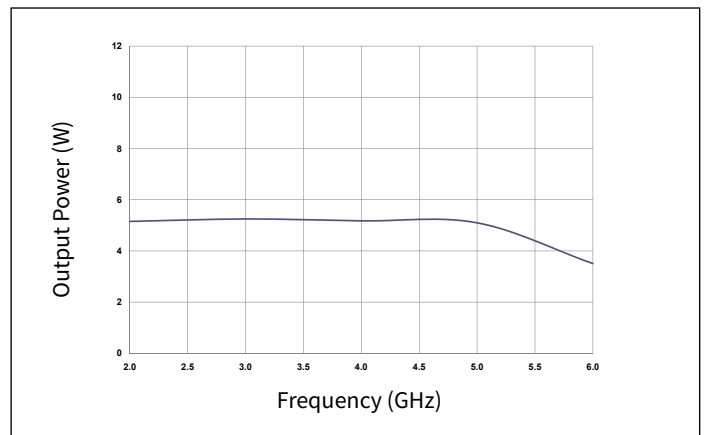
Figure 10. Output Power vs Frequency of the CGH40006P in the CGH40006P-AMP P_{IN} = 30 \text{ dBm} , V_{DD} = 20 \text{ V}
