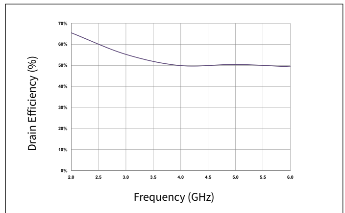
Figure 12. Drain Efficiency vs Frequency of the CGH40006P in the CGH40006P-AMP P_{IN} = 30 \text{ dBm} , V_{DD} = 20 \text{ V}
