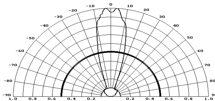
Directive Characteristics
