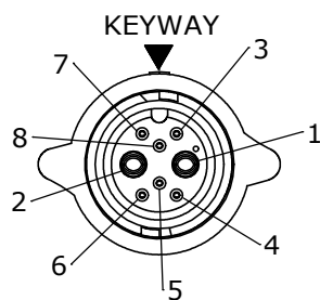
END "A" FACE VIEW
