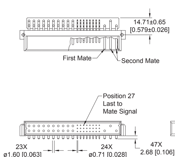
CONNECTOR DIMENSIONS
