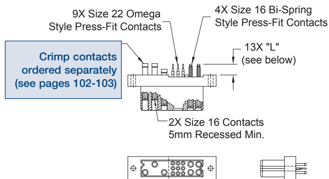
CONNECTOR DIMENSIONS
