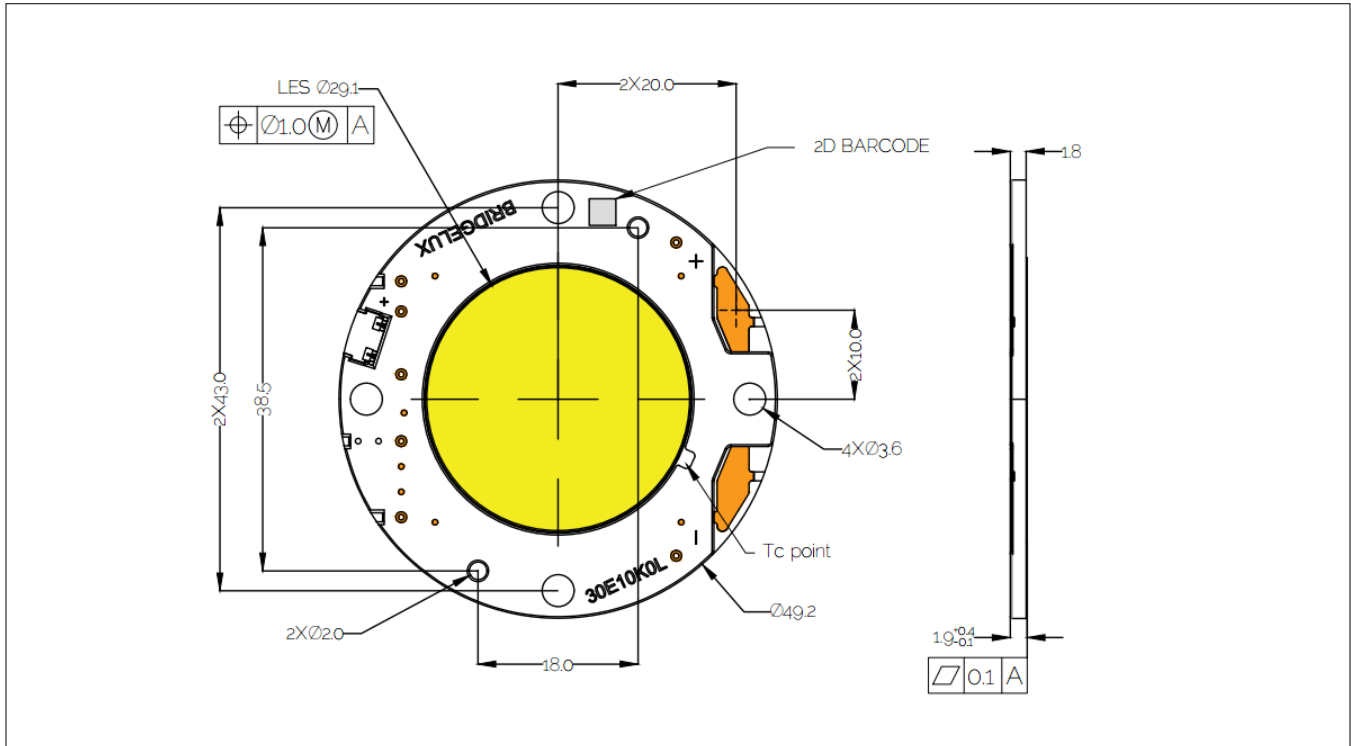
Figure 22: Drawing for Vero 29 LED Array
