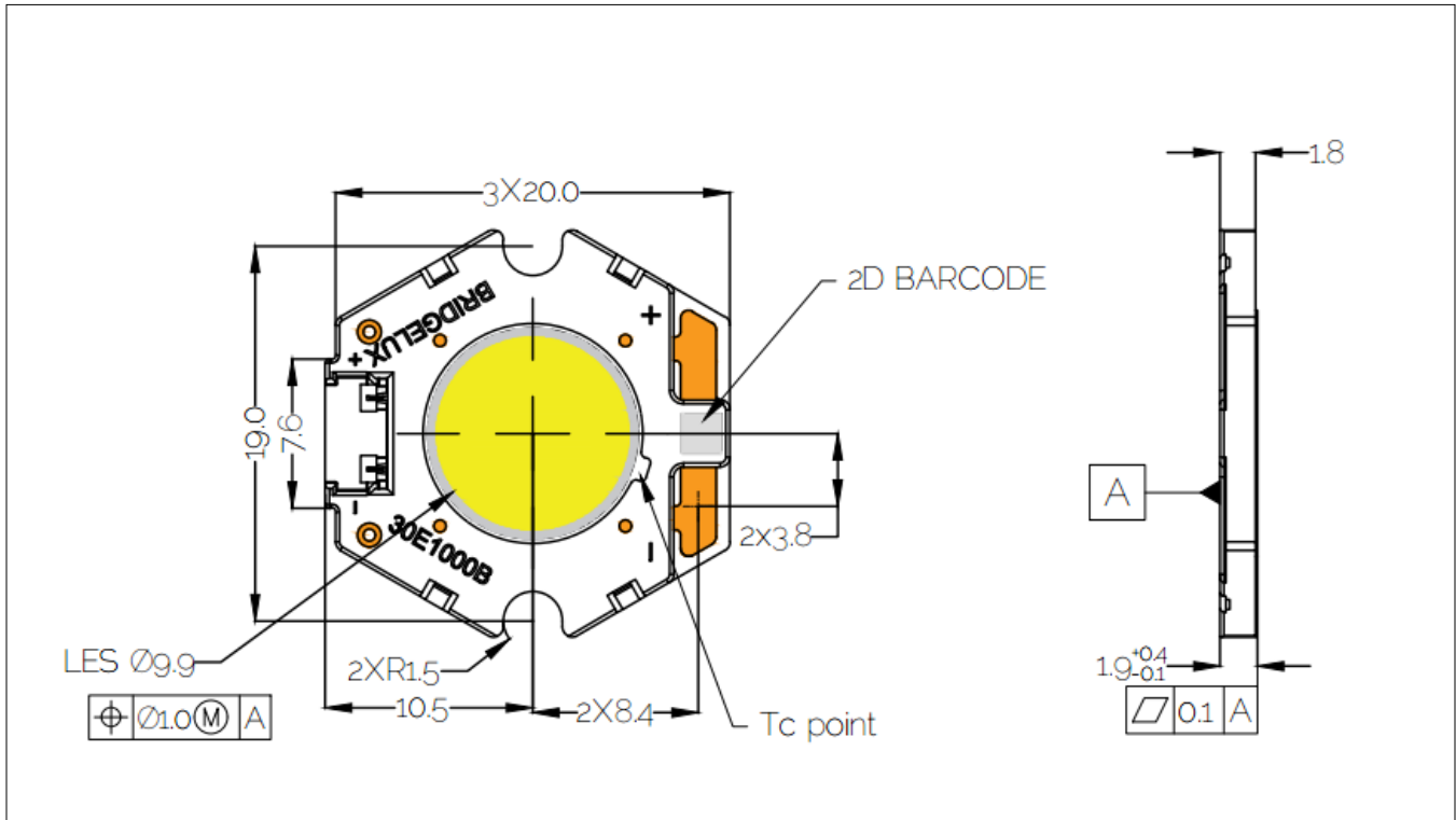
Figure 21: Drawing for Vero 10 LED Array
