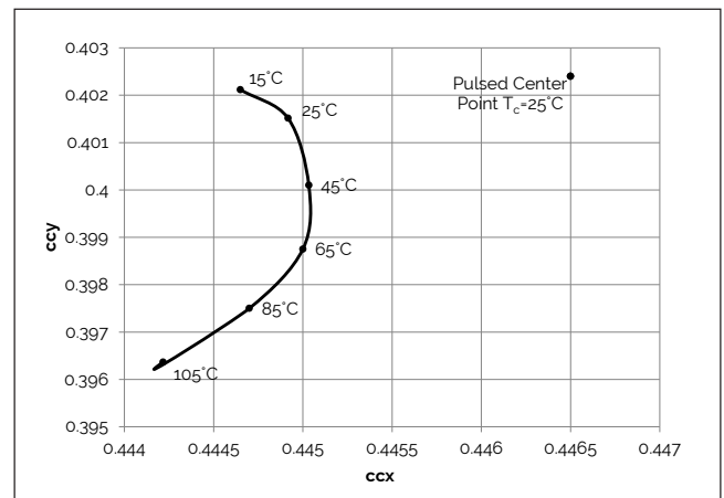
Figure 11: 3000K, 90 CRI Color Shift vs. Case Temperature 3
