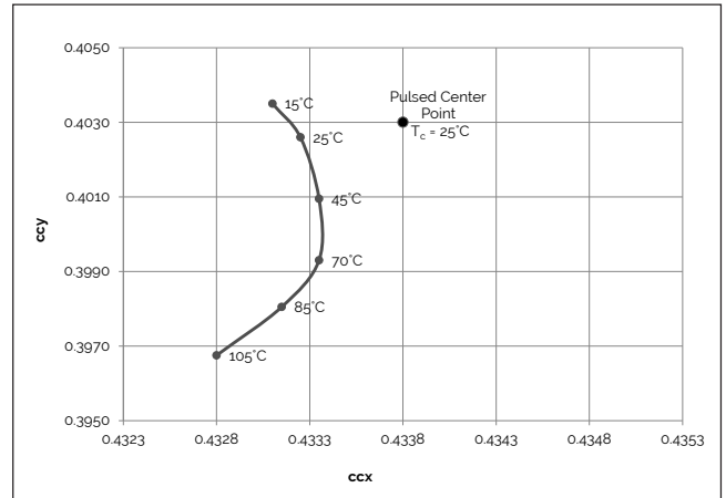
Figure 9: 3000K, 97 CRI Color Shift vs. Case Temperature 1
