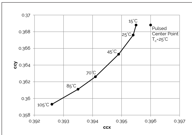
Figure 10: 3500K Class A Color Shift vs. Case Temperature 1
