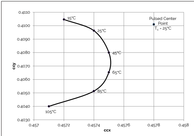
Figure 8: 2700K, 97 CRI Color Shift vs. Case Temperature 1
