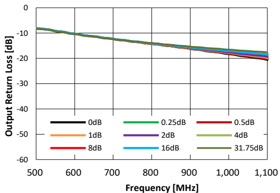
Figure 14. Output Return Loss vs. Frequency over Major Attenuation States
