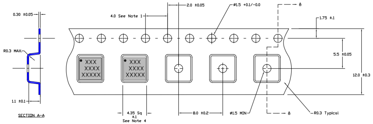
Figure 96. Tape & Reel
