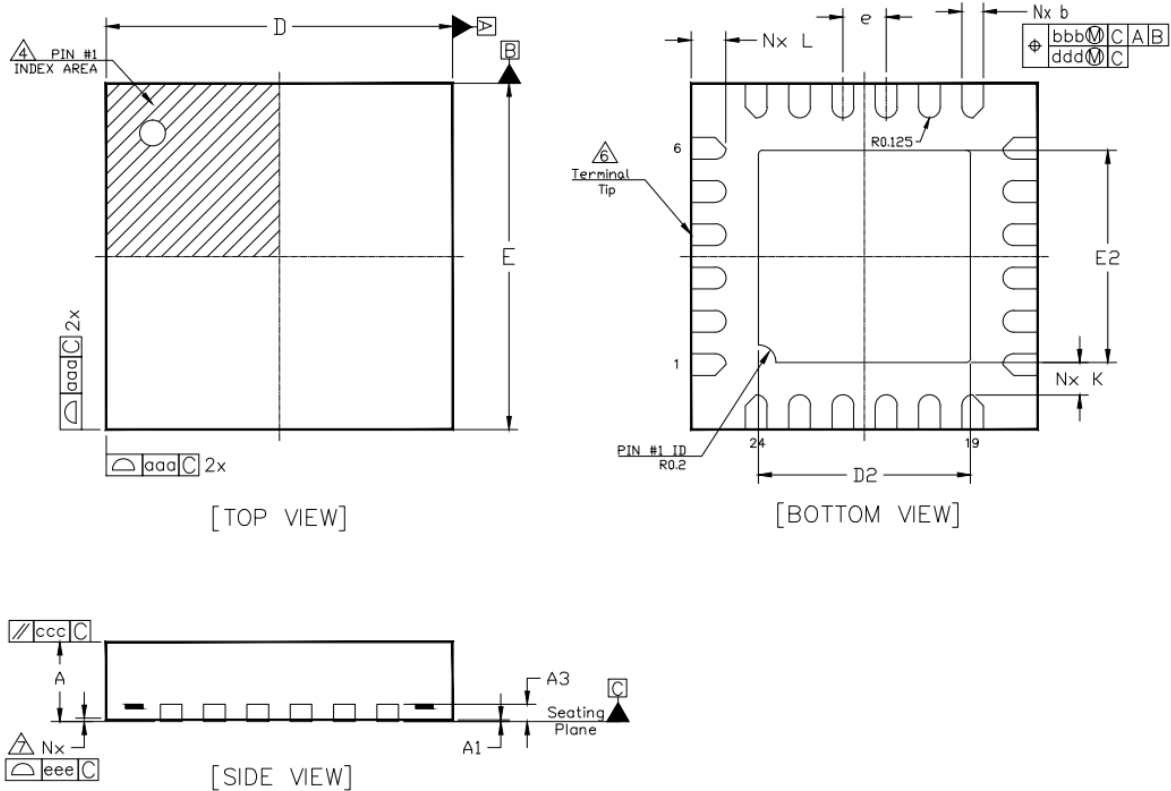
Figure 95. Package Outline Dimension
