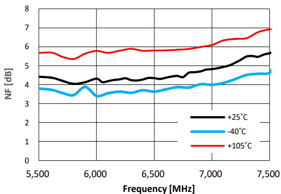
Figure 85. Noise Figure vs. Frequency @ VDD = 5V Over Temperature (Max Gain State)
