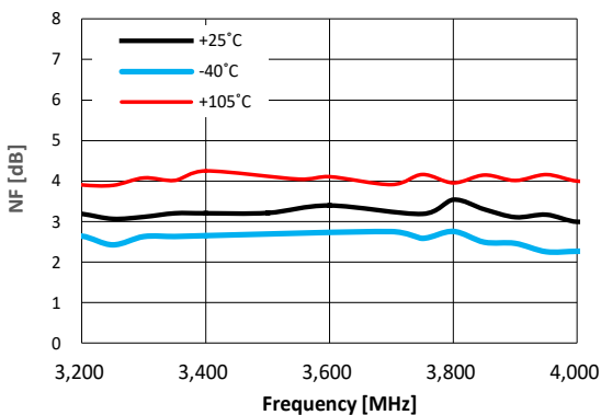
Figure 51. Noise Figure vs. Frequency @ VDD = 5V Over Temperature (Max Gain State)
