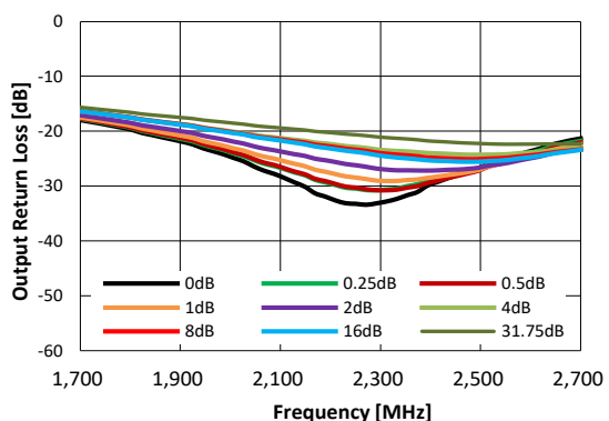
Figure 31. Output Return Loss vs. Frequency over Major Attenuation States
