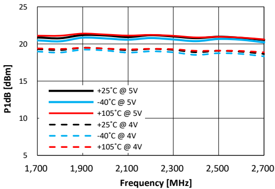
Figure 33. P1dB vs. Frequency vs. VDD Over Temperature (Max Gain State)
