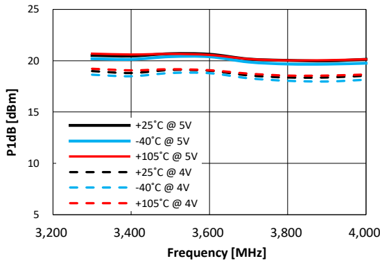
Figure 50. P1dB vs. Frequency vs. VDD Over Temperature (Max Gain State)
