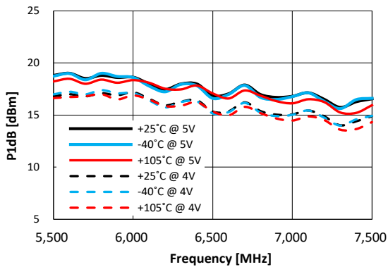
Figure 84. P1dB vs. Frequency vs. VDD Over Temperature (Max Gain State)
