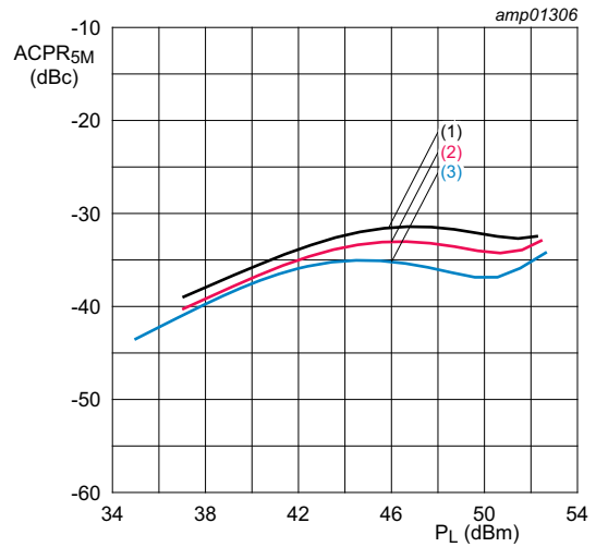
V_{DS} = 30\text{ V}; I_{Dq} = 800\text{ mA}; V_{GS(amp)peak} = 1.1\text{ V}. (1) f = 1805\text{ MHz} (2) f = 1845\text{ MHz} (3) f = 1880\text{ MHz}
