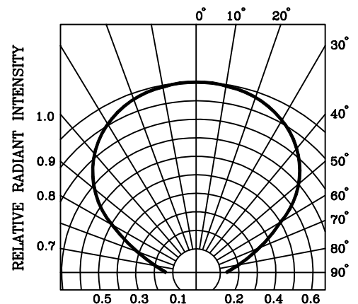
Fig.6 RADIATION DIAGRAM
