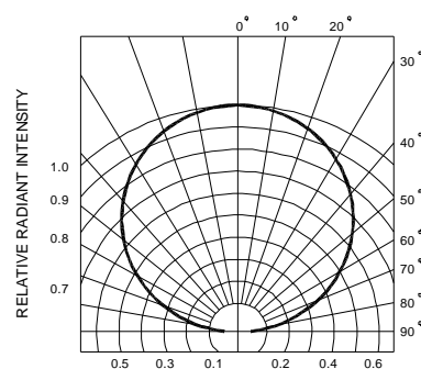
RADIATION DIAGRAM
