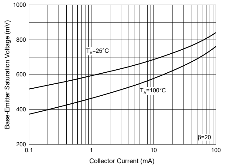
Fig. 4 - Base-Emmitter Saturation Voltage Characteristics
