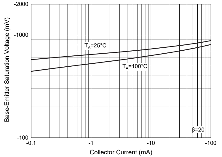
Fig. 10 - Base-Emitter Saturation Voltage Characteristics
