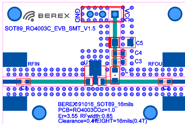
PCB Mounting
